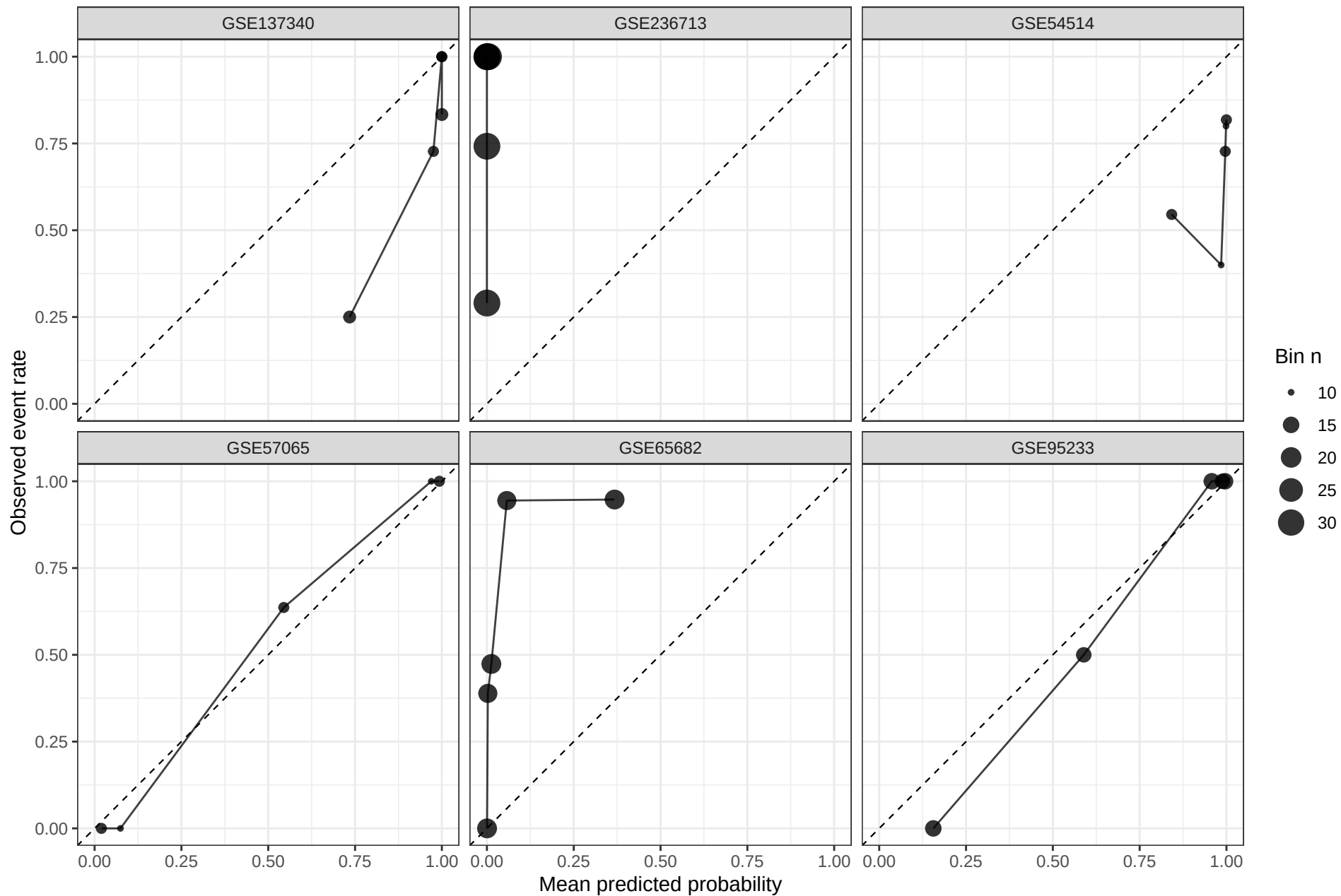
LODO calibration plots by validation dataset
