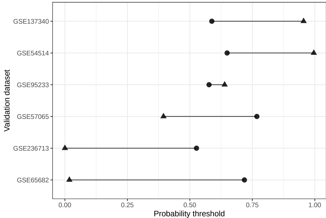
Threshold drift across LODO validation datasets
