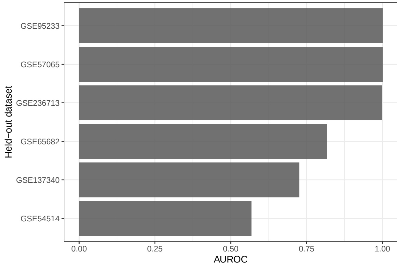
Nested LODO validation AUROC
