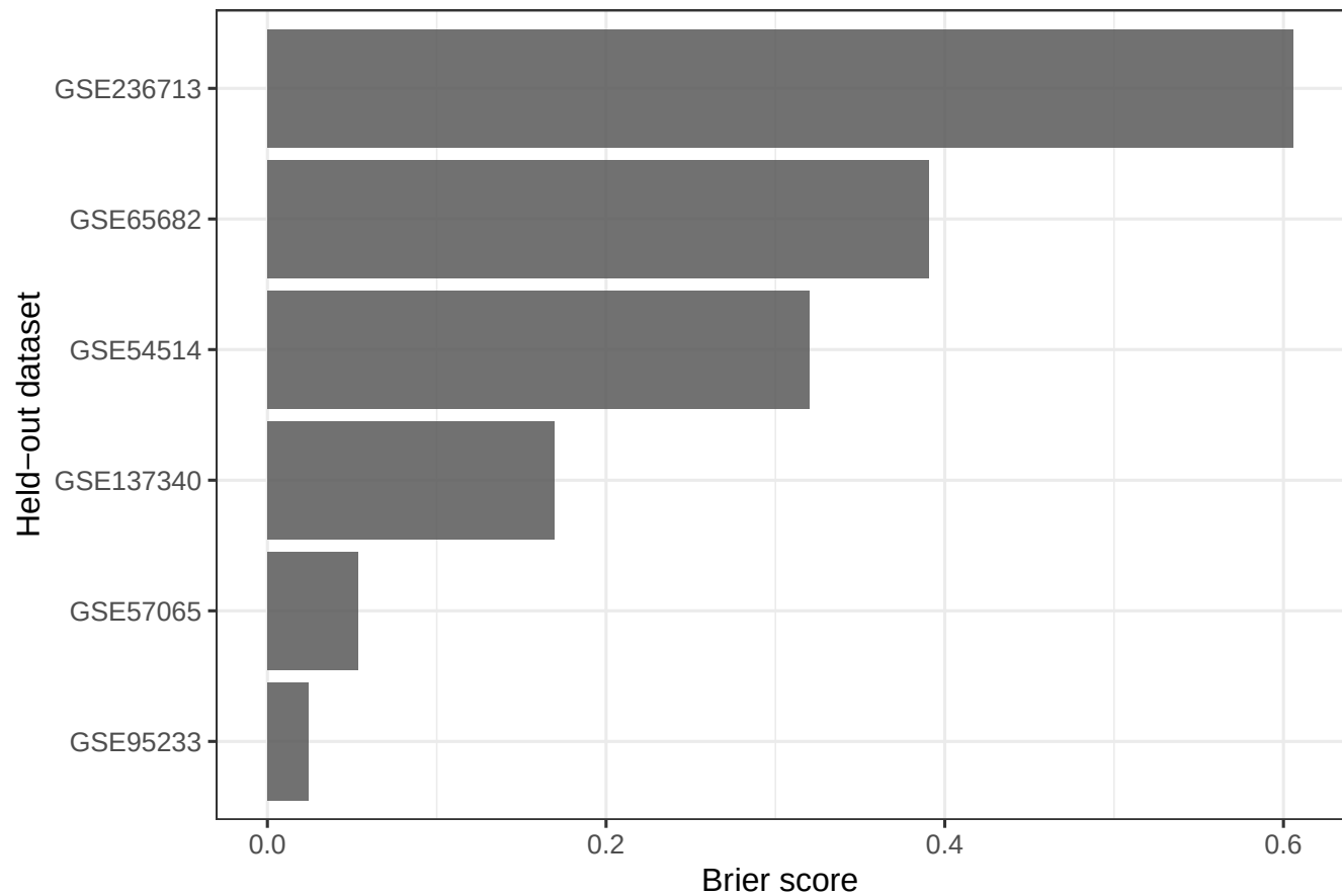
Nested LODO validation Brier score
