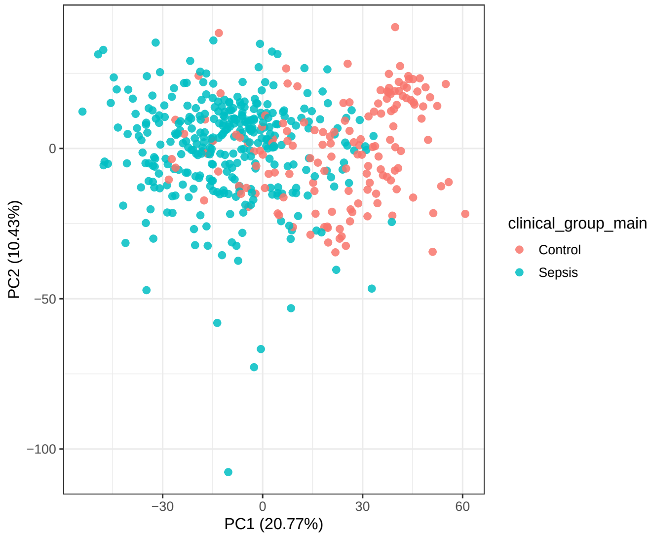
PCA of ComBat-adjusted expression by group
