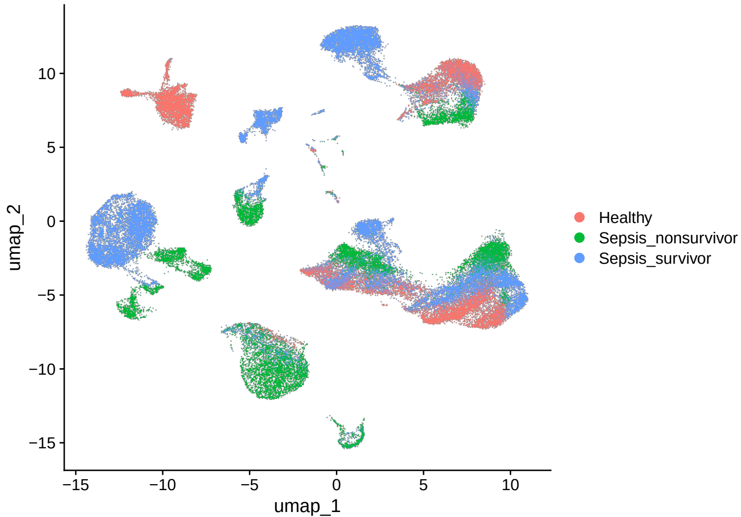
GSE167363 UMAP by clinical group
