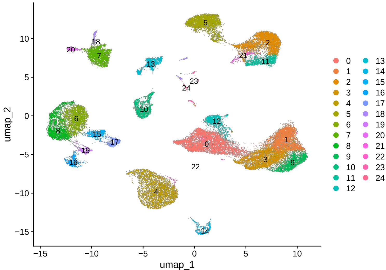
GSE167363 UMAP by Seurat cluster
