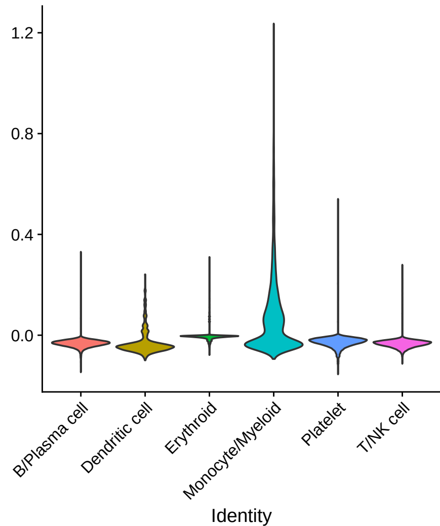
MyeloidInnateUp_score
