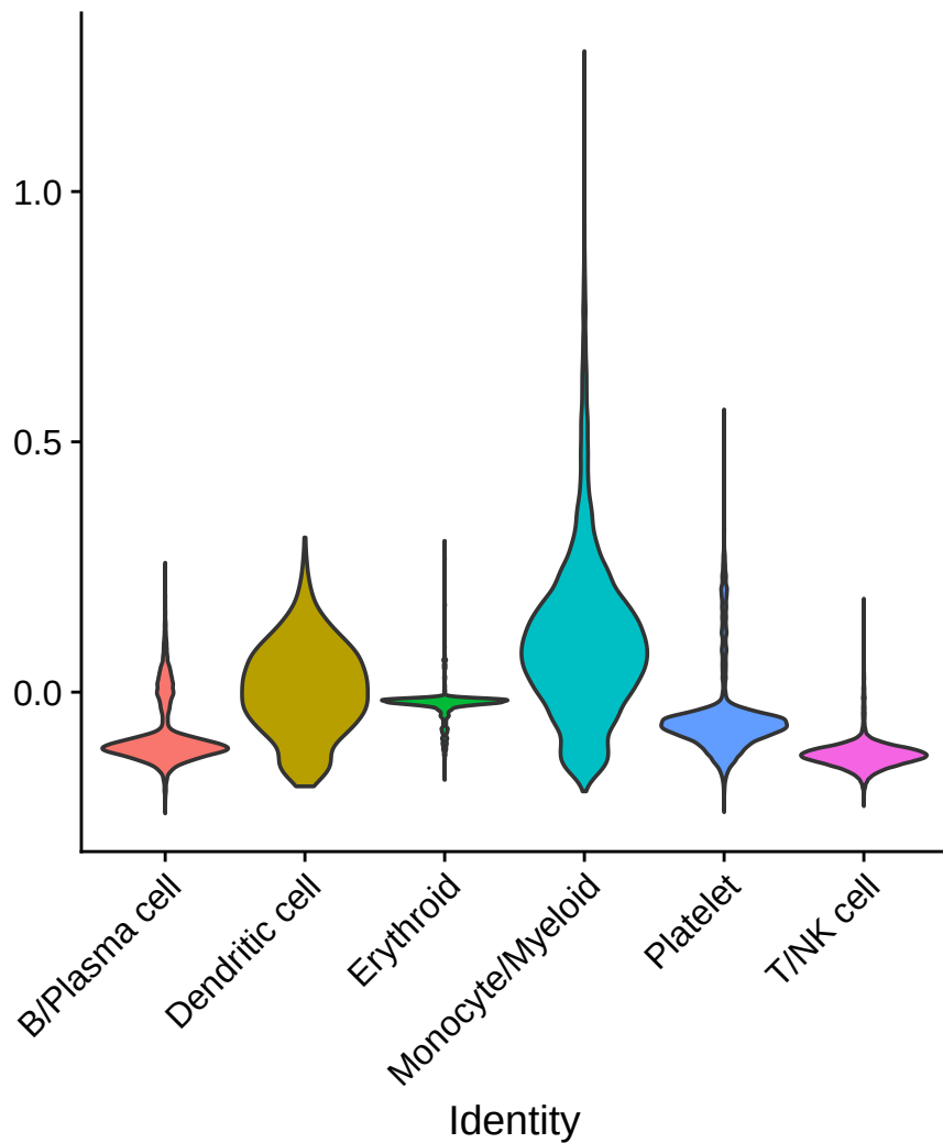
Final10_score
