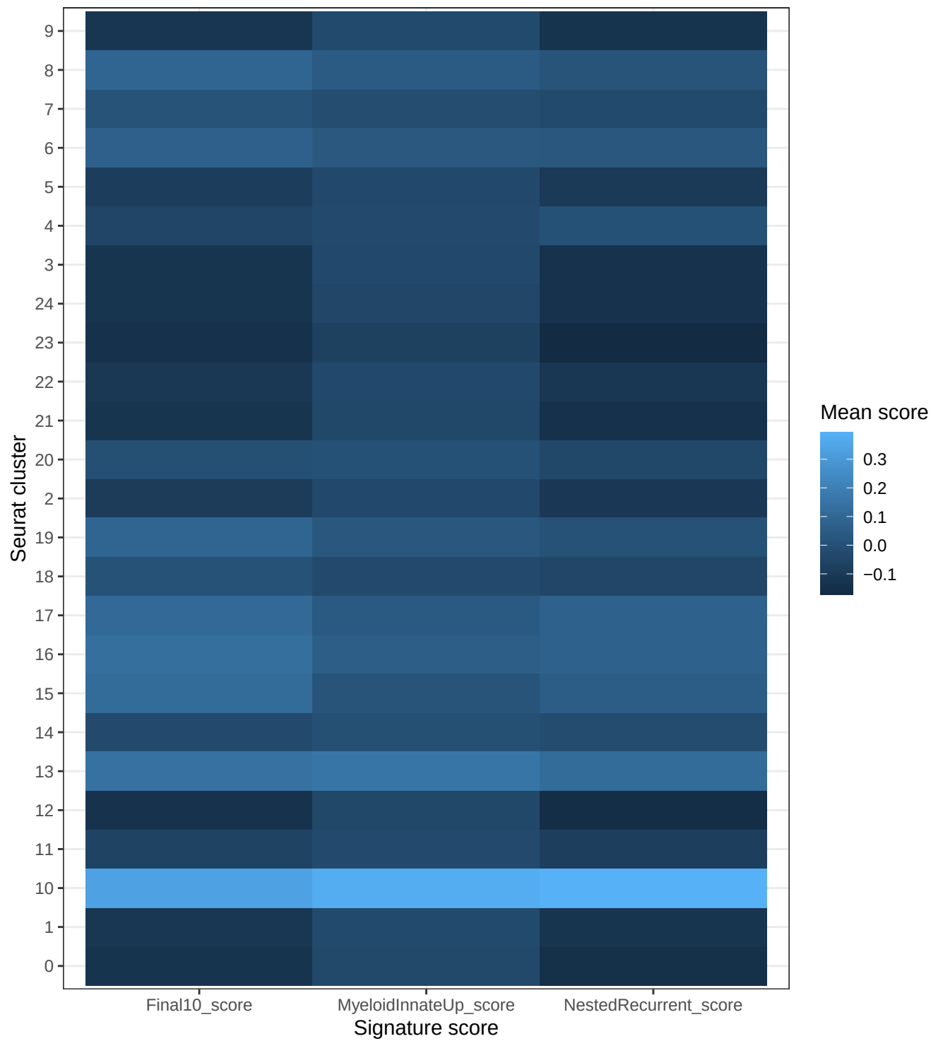
Signature module scores by Seurat cluster
