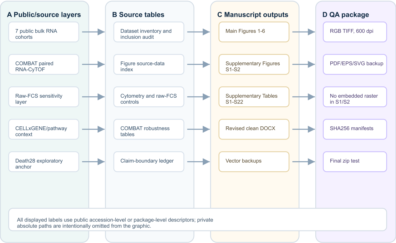
Supplementary Figure S2. Data-source and reproducibility traceability map. Schematic links public/source layers to figure outputs, QA checks, checksums and the upload-ready package.
