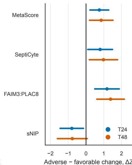
E GSE57065, baseline SAPS II category
