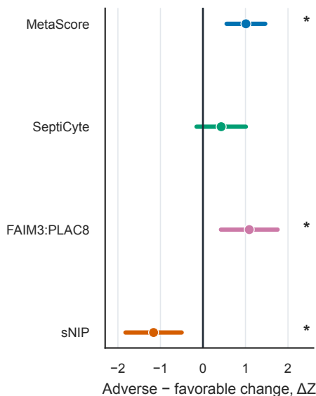
D GSE110487, organ-function course
