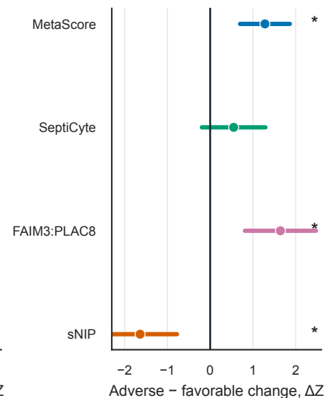
F GSE54514, source-defined survival
