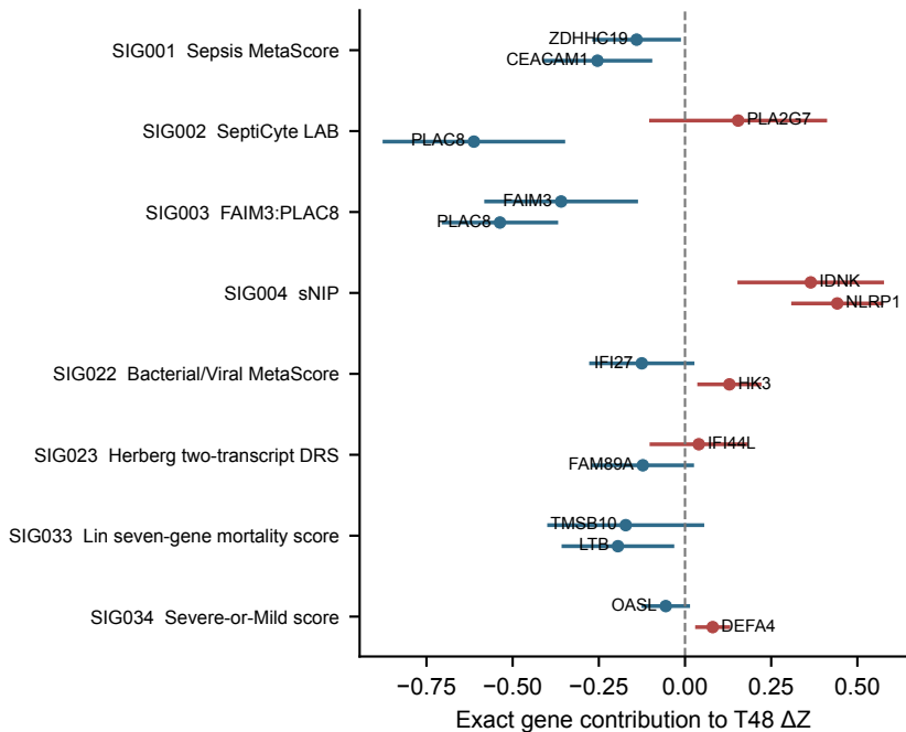
a Two largest pooled mathematical contributions
