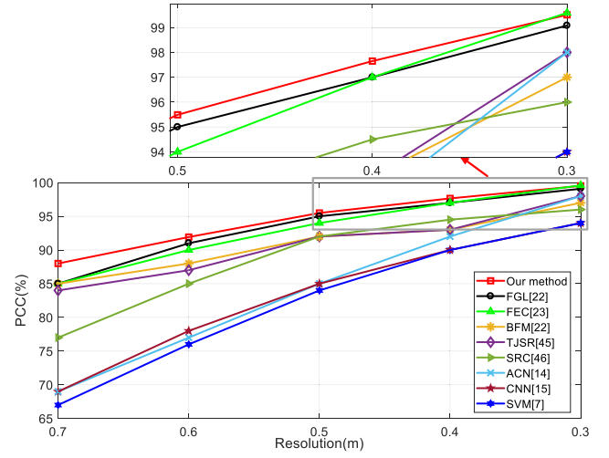
Fig. 11. Test PCCs of different methods for the test images under different resolutions (EOC-3).
