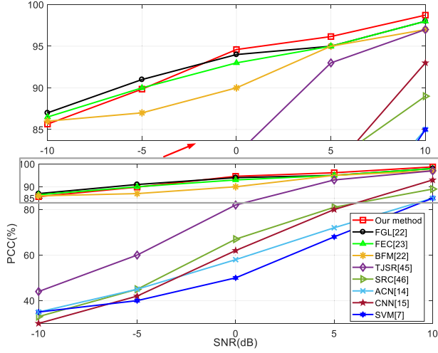
Fig. 9. Test PCCs of different methods under different SNRs (EOC-2).
