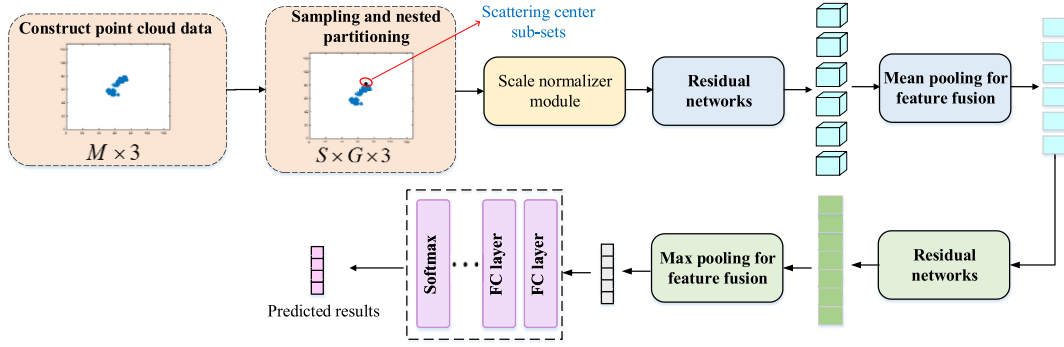
Fig. 3. Architecture of the target recognition module in our model.
