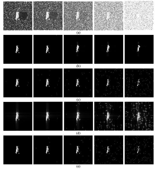
Fig. 8. Reconstructed images by different methods for SAR images under different SNRs. (a) Shows the noisy SAR images under SNRs being 10, 5, 0, -5, and -10 dB and (b)–(e) show the reconstructed images by our method, OMP, RELAX, and BCS algorithms, respectively.
