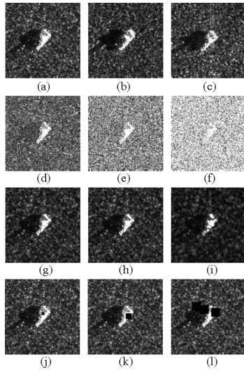
Fig. 5. SAR image samples of four EOC cases from T72 target. (a)–(c) are three versions of T72. (d)–(f) Show noised images for a sample from T72 with SNRs being 5, 0, and -5 dB, respectively. (g)–(i) Present the images with different resolutions for a sample from T72 with resolutions being 0.4 \times 0.4 m, 0.5 \times 0.5 m, and 0.6 \times 0.6 m, respectively. (j)–(l) Show the images with occlusions, and the cover sizes are 5 \times 5 , 10 \times 10 , and 15 \times 15 , respectively.
