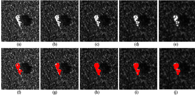
Fig. 10. Images with different resolutions and extracted scattering centers. (a)–(e) are the original images with resolutions being 0.3 \times 0.3 m, 0.4 \times 0.4 m, 0.5 \times 0.5 m, 0.6 \times 0.6 m, and 0.7 \times 0.7 m, respectively, and (f)–(j) show the corresponding extracted scattering centers by our model.
