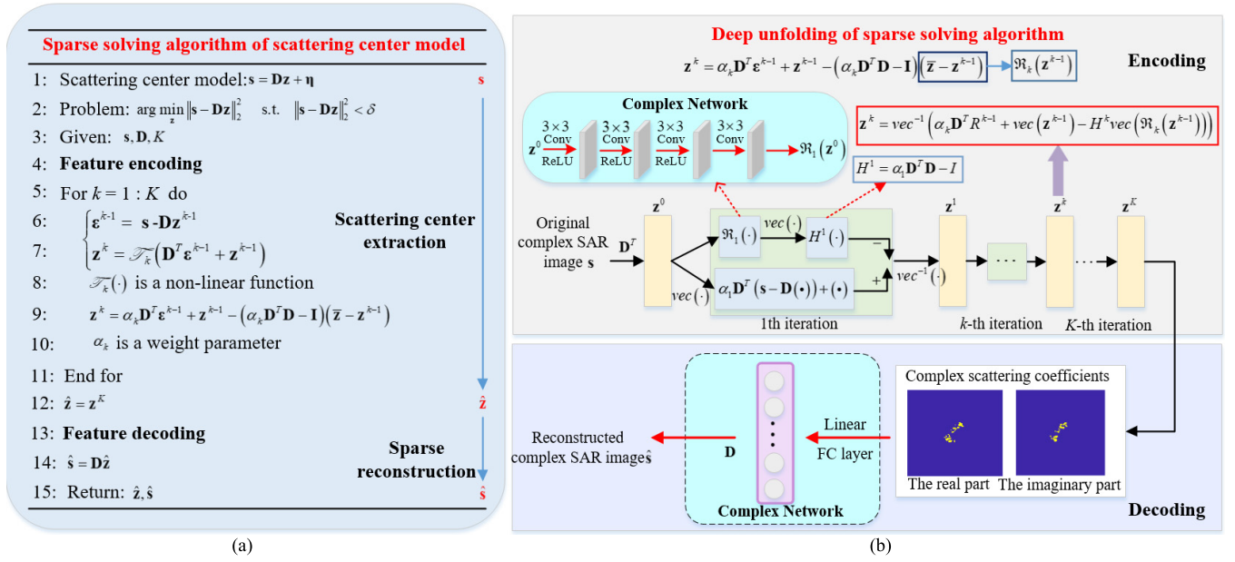
Fig. 2. Process of unfolding algorithm in our model. (a) AMP algorithm. (b) Architecture of the scattering center feature extraction module.
