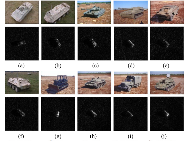
Fig. 4. Image examples of ten targets. The first row of (a)–(j) shows the optical images, and the second row of (a)–(j) shows corresponding SAR images. (a) BMP2, (b) BTR70, (c) T72, (d) 2S1, (e) BRDM2, (f) BTR60, (g) D7, (h) T62, (i) ZIL131, and (j) ZSU23/4.
