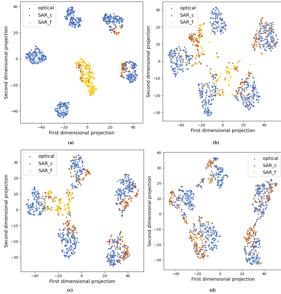
Fig. 8. t-SNE visualization of test split features generated by (a) “Source,” (b) “DANN,” (c) “DSAN,” and (d) proposed approach (ours), where different colors are used to distinguish different situations. Red represents features of correctly aligned SAR images, yellow represents features of falsely aligned SAR images, and blue represents features of optical images.
