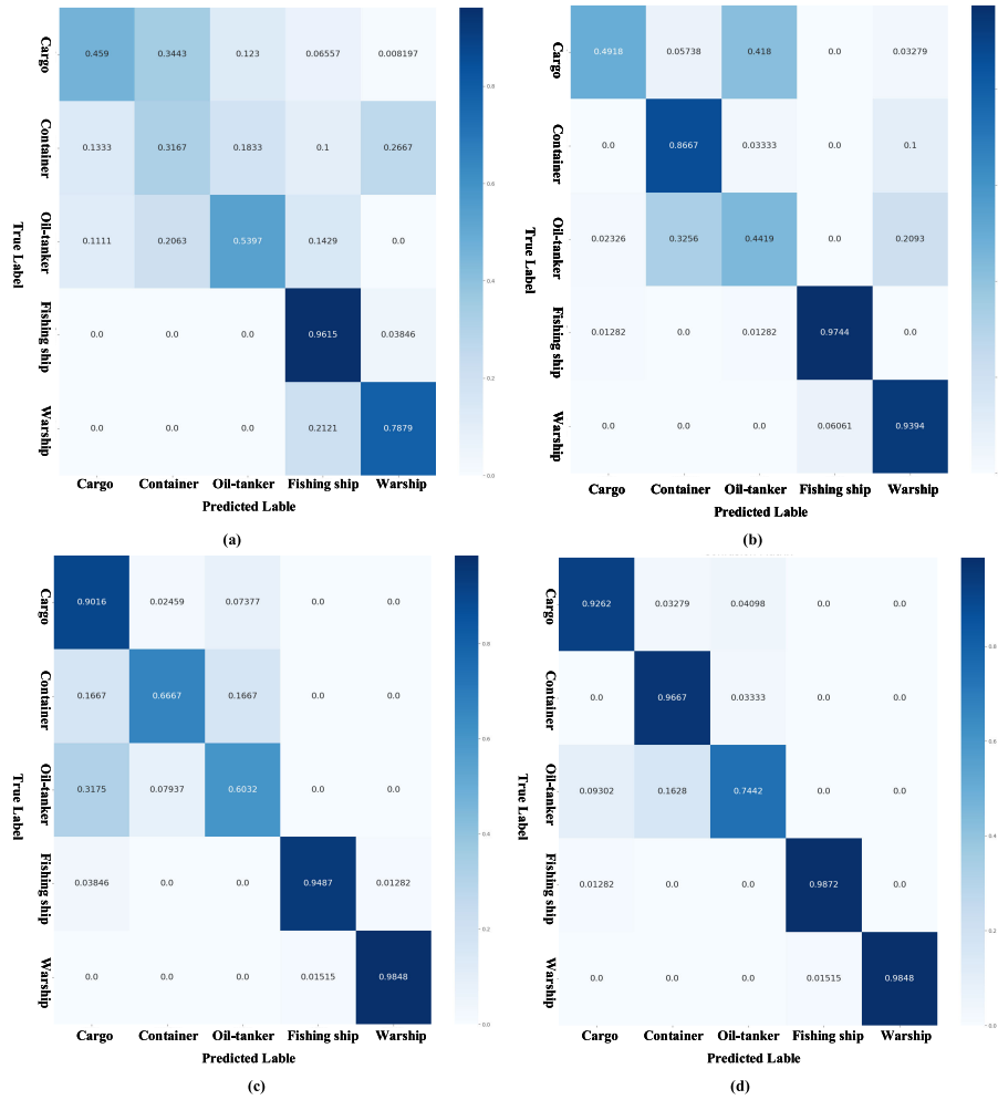
Fig. 9. Confusion matrix of the different methods. (a) DANN. (b) DSAN. (c) Ours. (d) Supervised.
