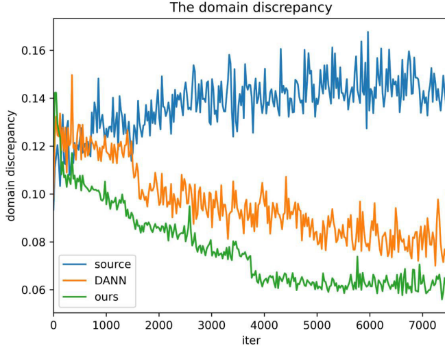
Fig. 11. Domain discrepancy of different methods as the number of iterations changes.
