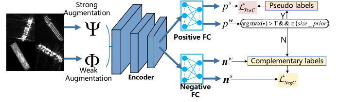
Fig. 4. Illustration of the proposed consistency enhancement learning. For unlabeled SAR images, we divide them into two parts according to their confidence and size prior: samples with pseudo-labels and samples with complementary labels. For pseudo-labels, we enforce the output of the positive classifier from different perturbed versions to be consistent. For complementary labels, we enforce consistency regularization on negative classifier with soft labels of different perturbed versions.
