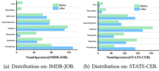
Figure 9: Diagnostic: Operator Distribution Shift.
