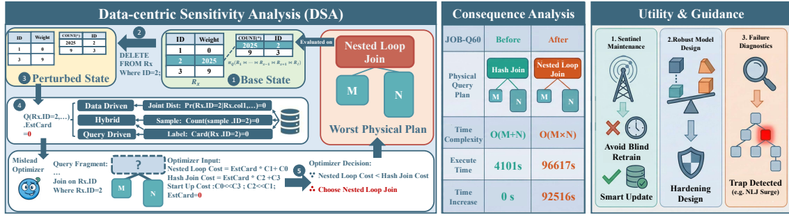
Figure 2: The Data-centric Sensitivity Analysis (DSA) Ecosystem. Illustrating the process of auditing worst-case data drifts (Left), quantifying their impact on query execution (Middle), and leveraging these insights for robust system guidance (Right).
