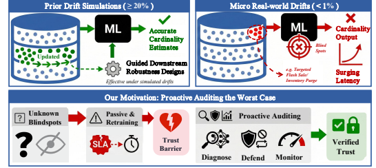
Figure 1: From Passive Simulations to Proactive Auditing.
