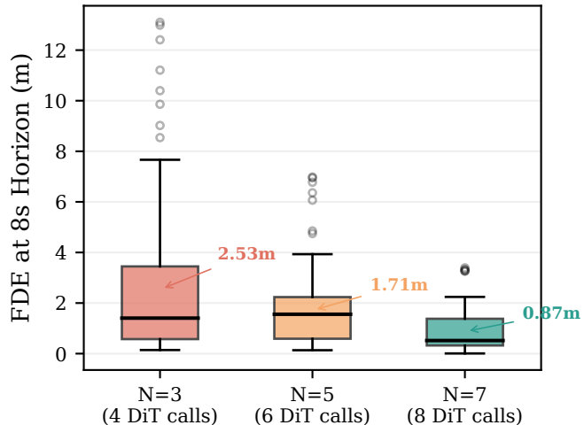
(a) Step-Count Sensitivity (131 frames)
