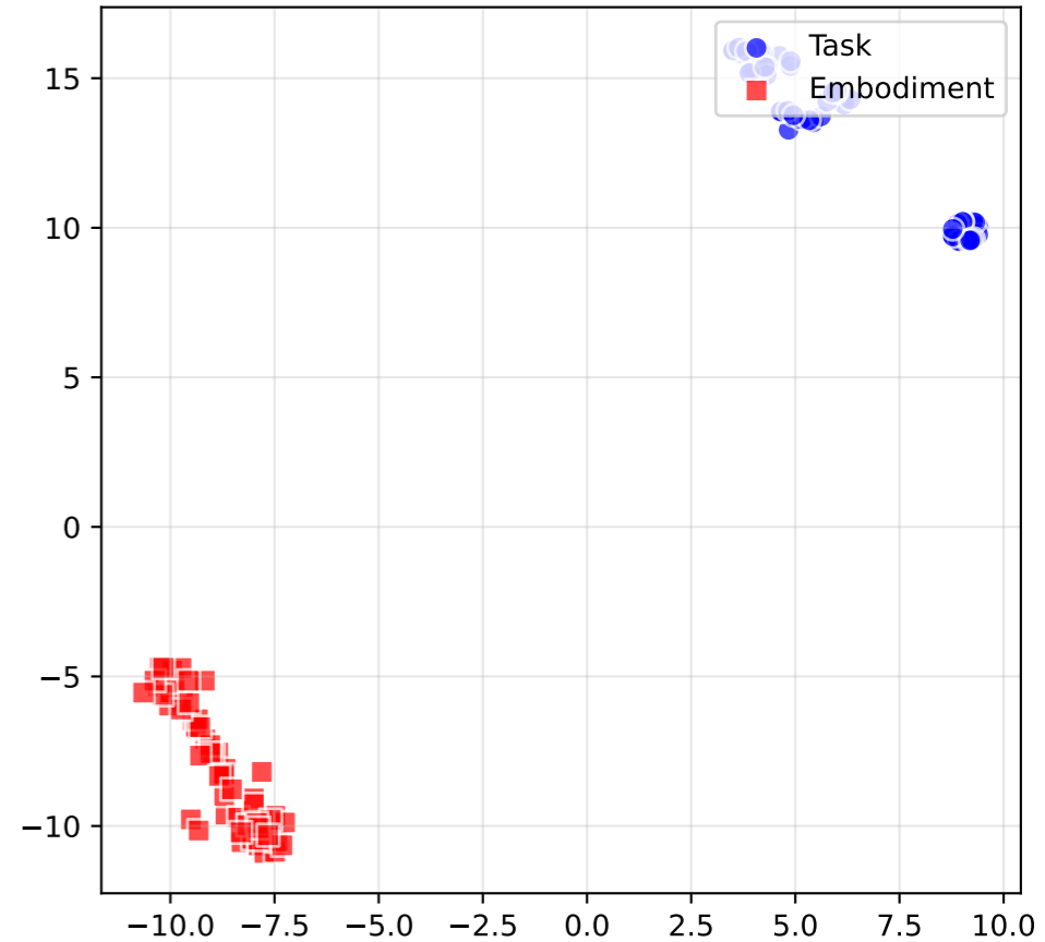
Combined Space
