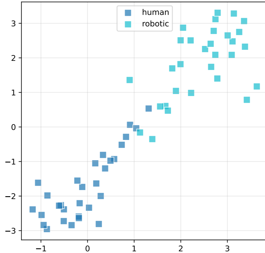
Embodiment Space
