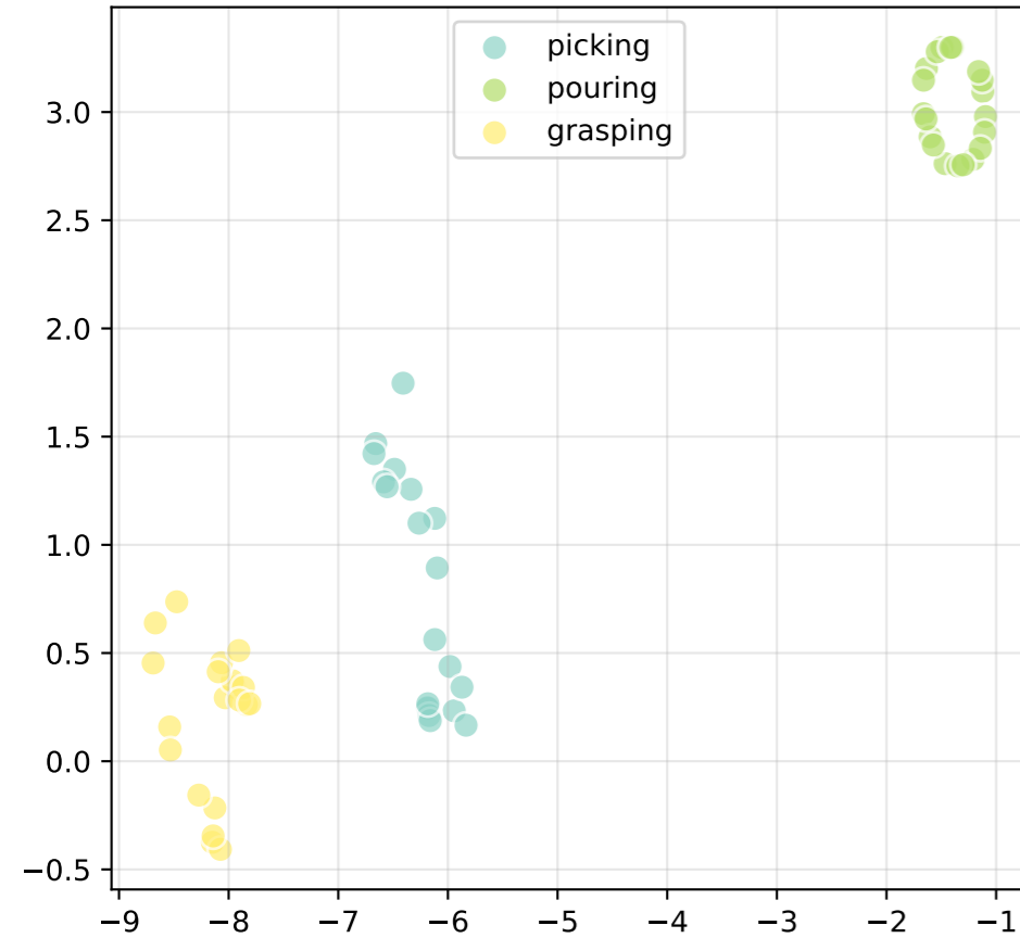
Task Space
