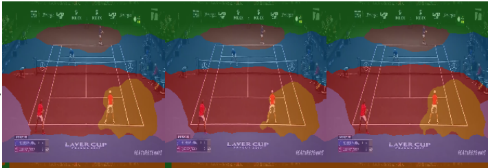
Grounded Correspondence
