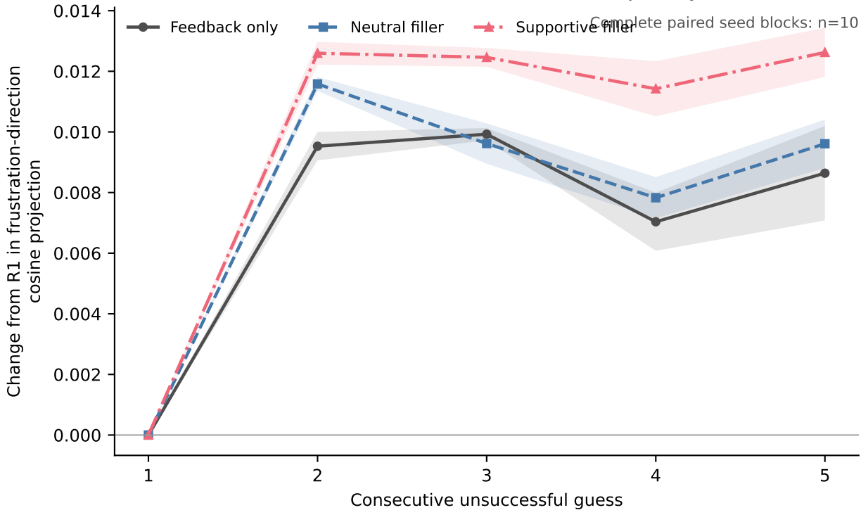
Five-round frustration-direction trajectory
