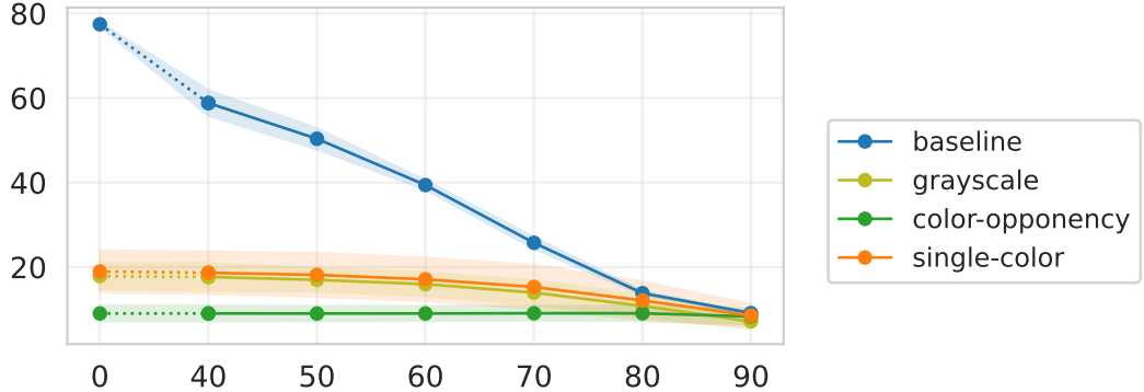
Mask2Former
