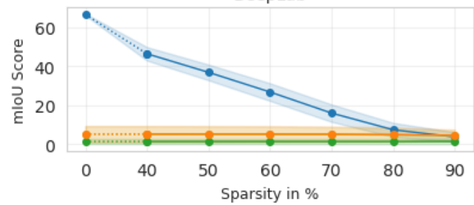
DeepLab
