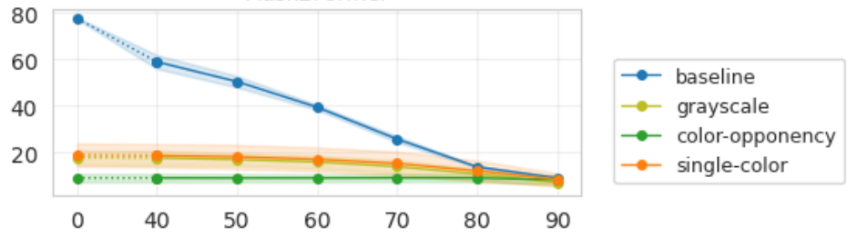
Mask2Former
