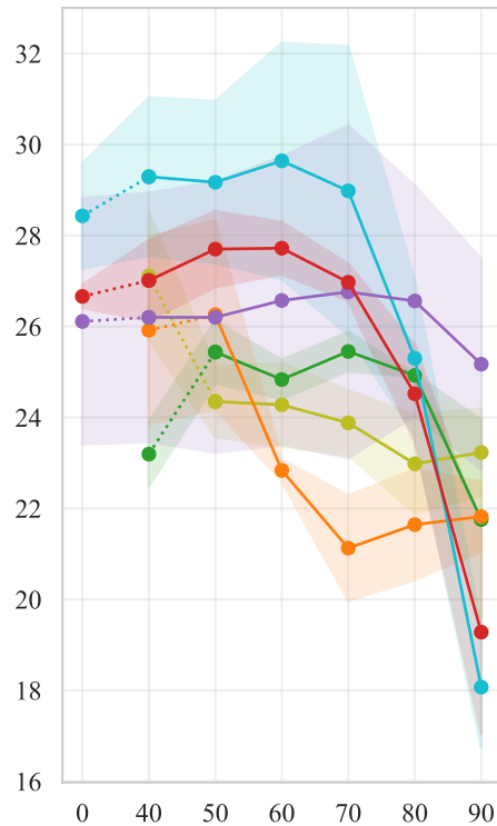
ACDC-night
