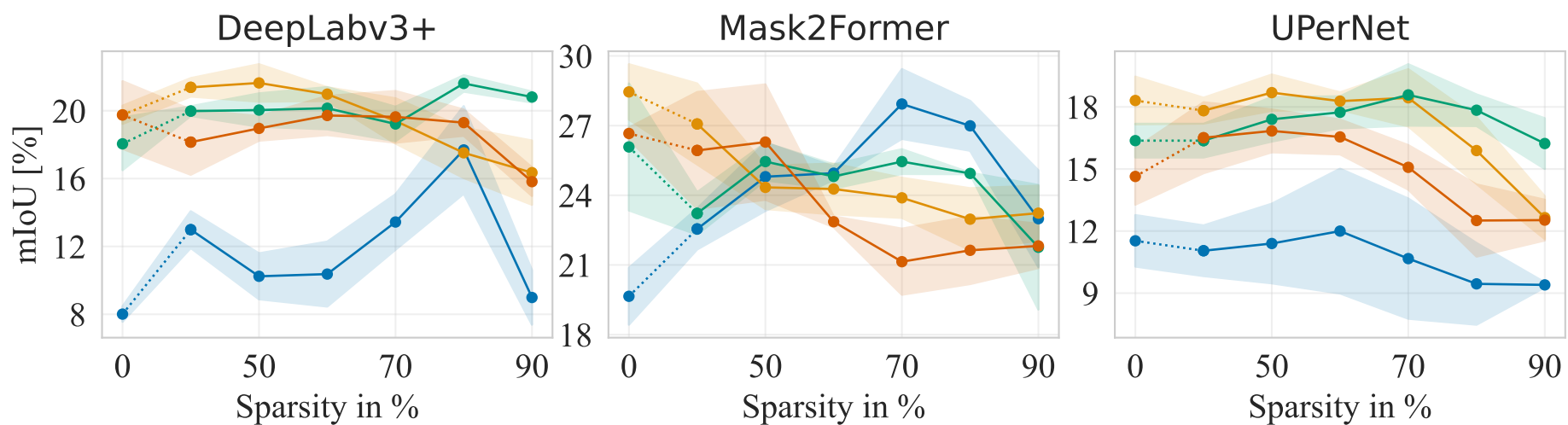
ACDC Night
