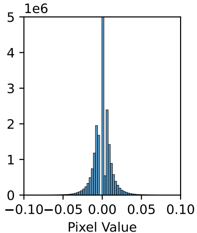
Sparse Image (0.7)
