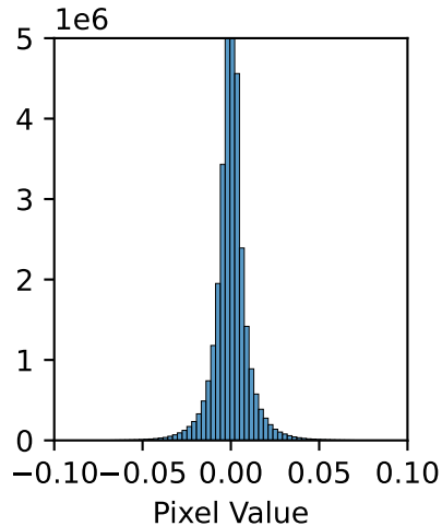
Preprocessed Image
