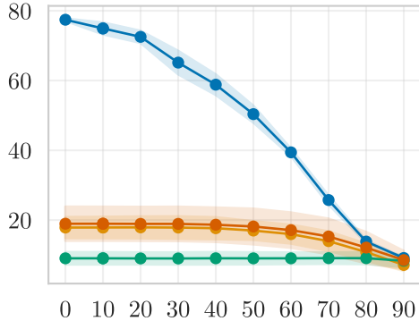
Mask2Former
