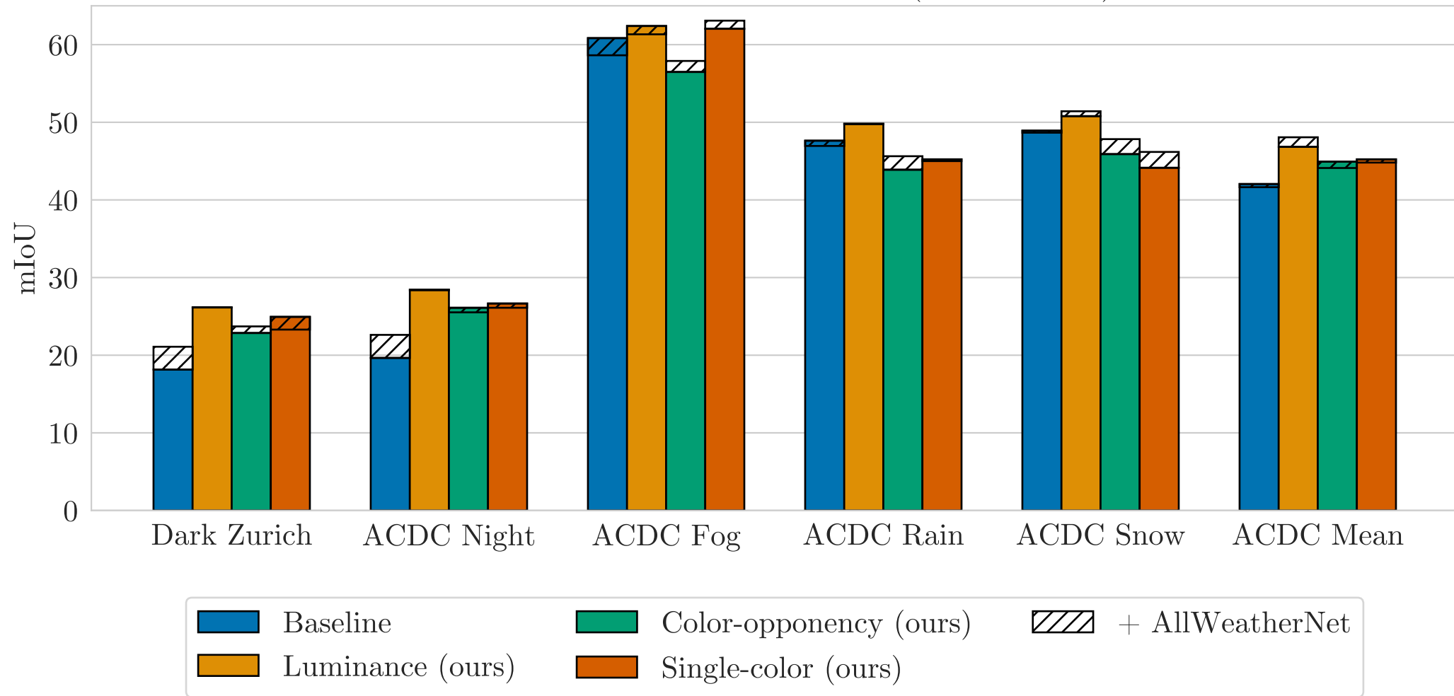
Base mIoU + AllWeatherNet Gain (Stacked View)
