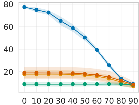
Mask2Former
