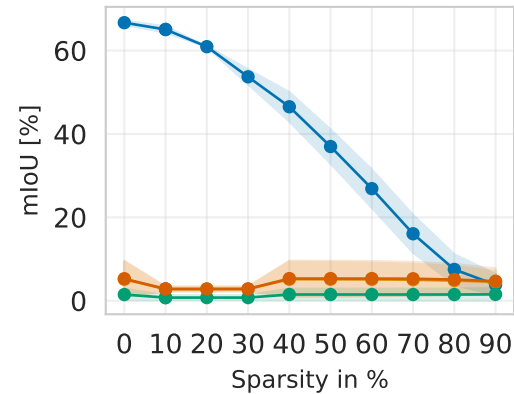
DeepLabv3+
