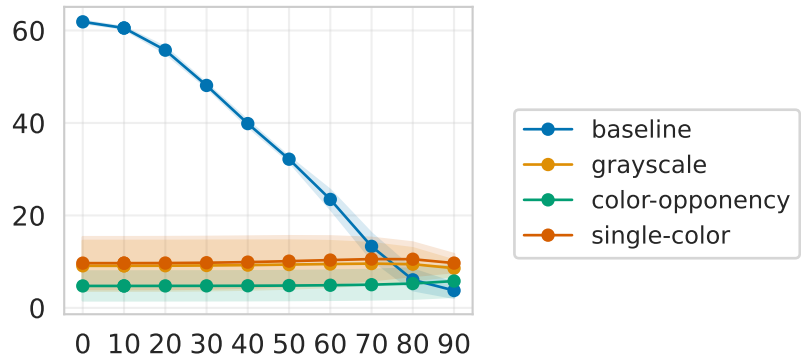
InternImage
