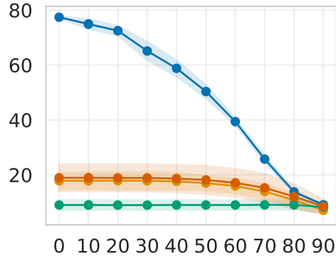
Mask2Former
