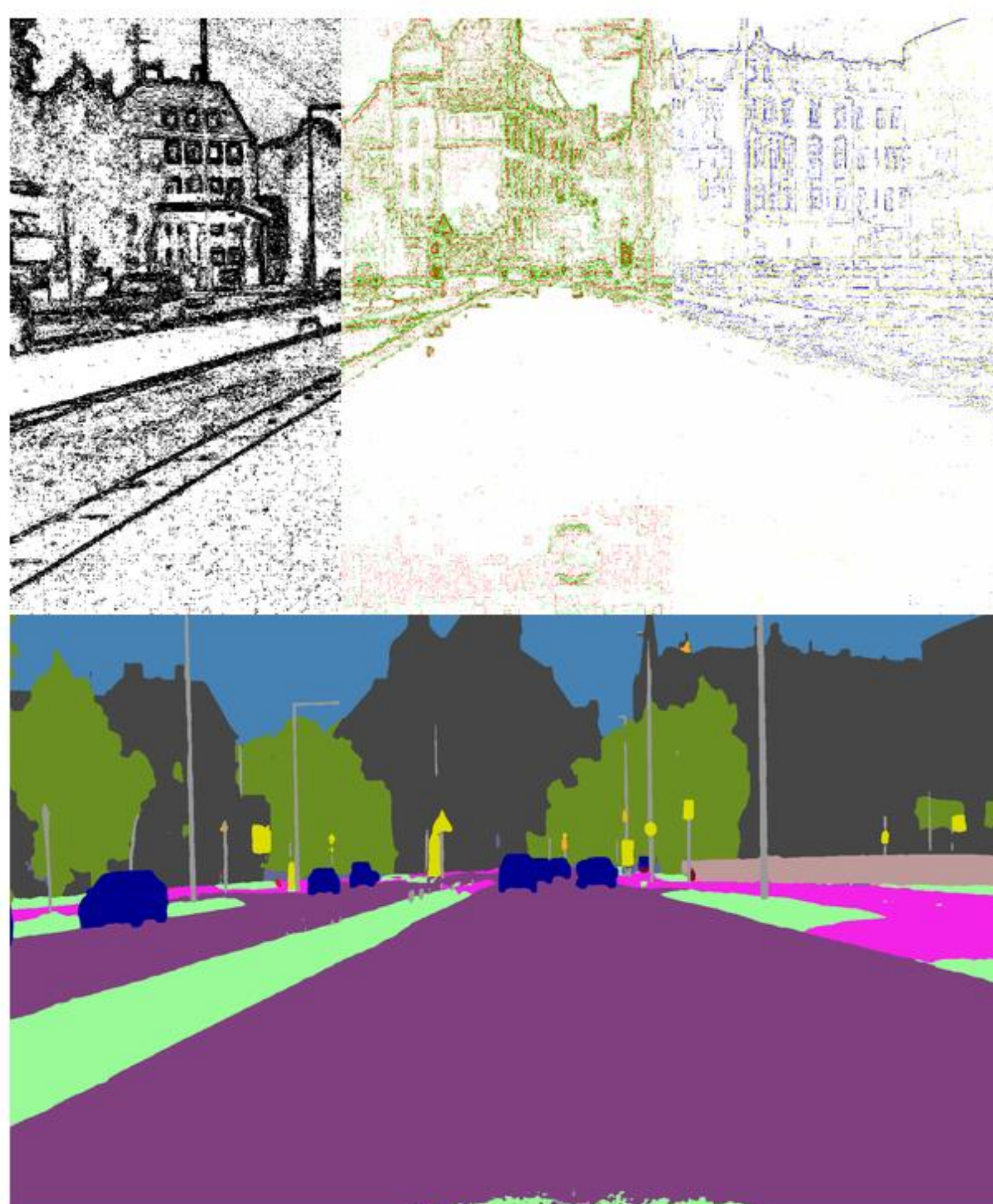
Color-opponency
