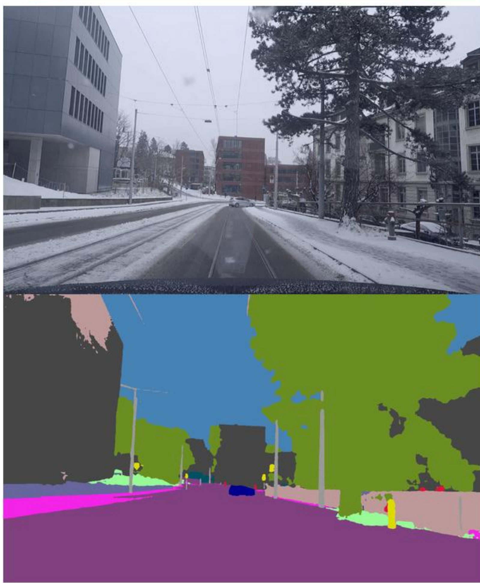
ACDC Snow
