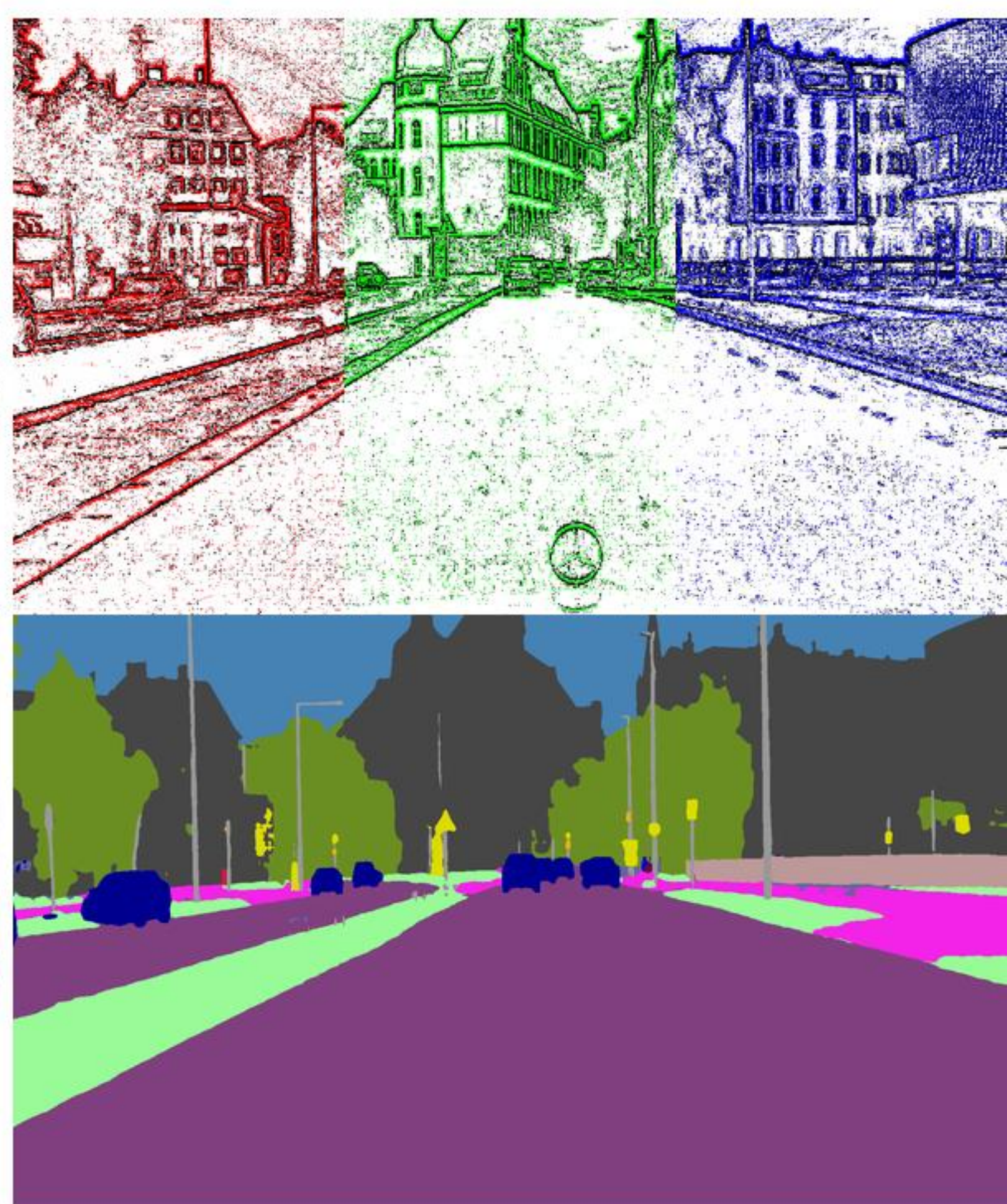
Single-color
