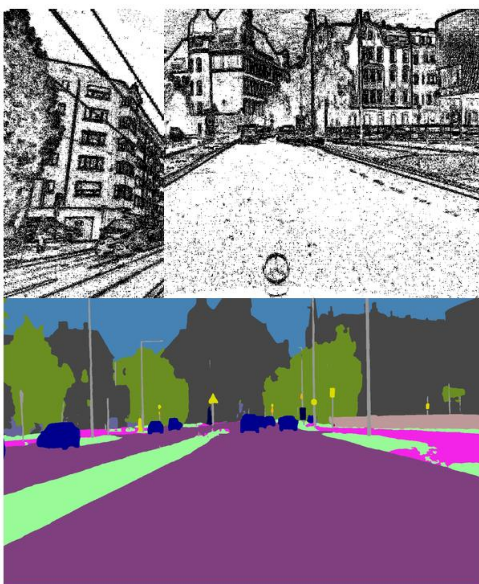
Luminance
