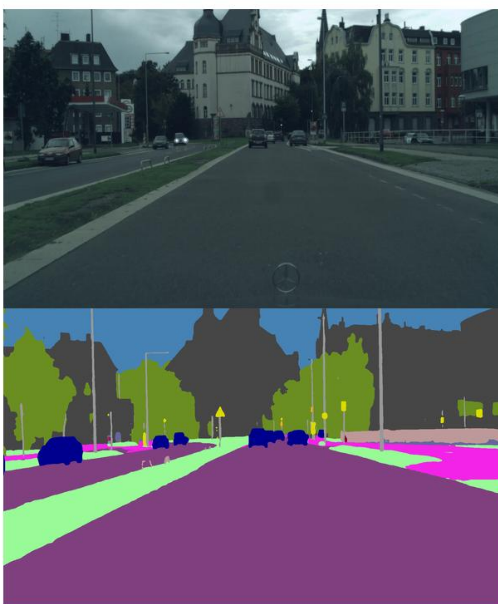
Original Image
