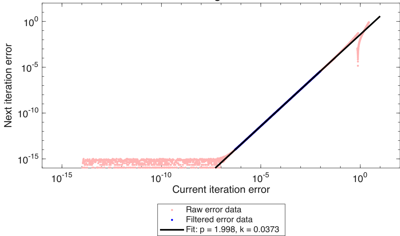
Newton Convergence: 1000 Trials
