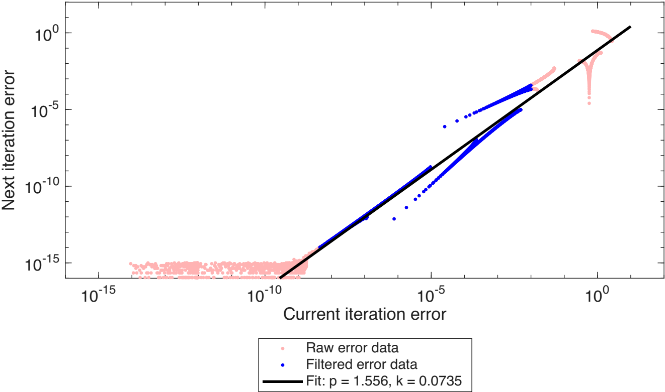
Secant Convergence: 1000 Trials
