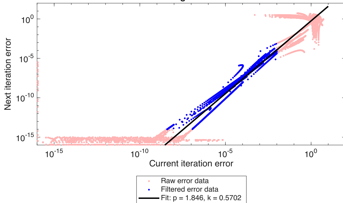
fzero Convergence: 1000 Trials
