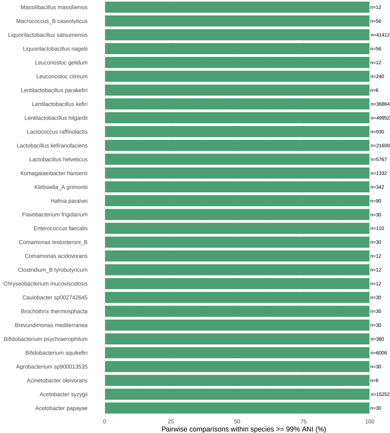
Supplementary Fig. 5. Per-species proportion of within-species MAG pairs reaching \geq 99\% ANI.
