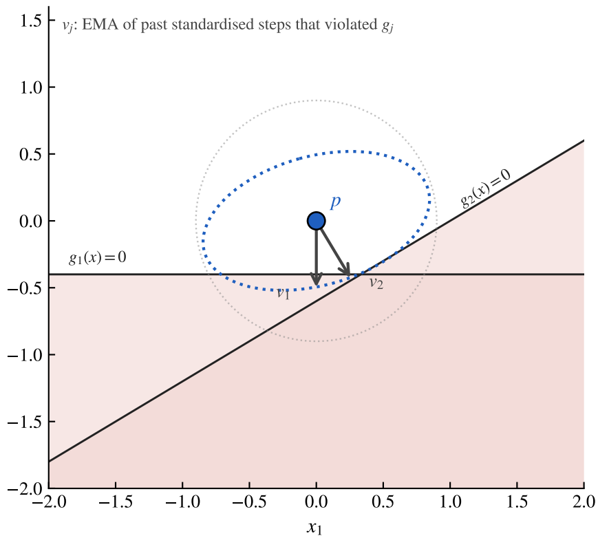
After many generations: v_j EMA and squeezed C'
