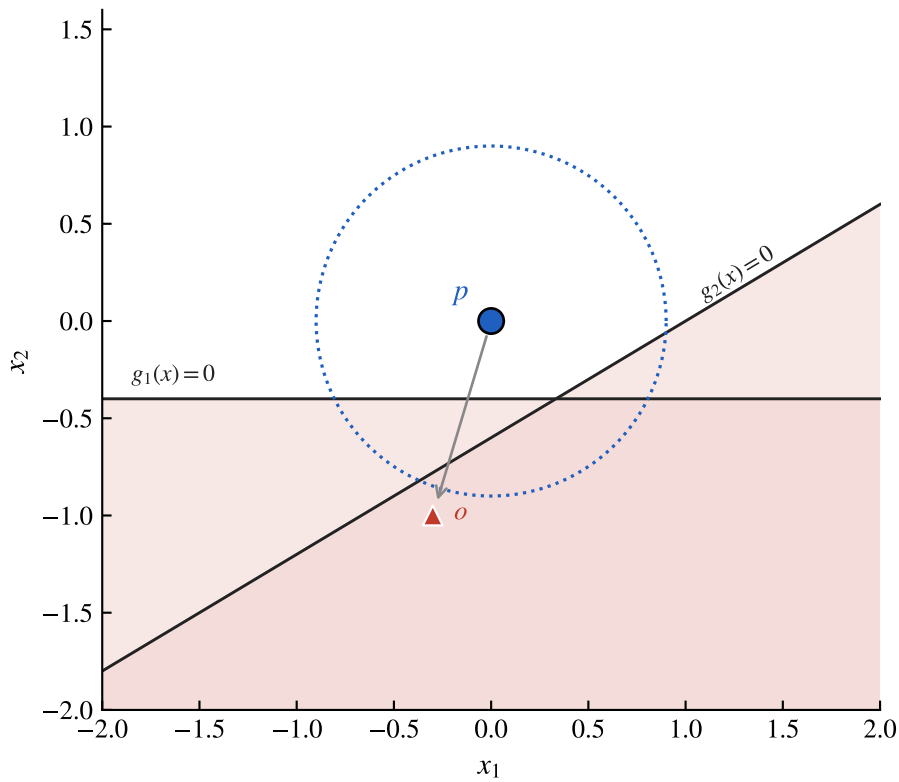
Generation 1: first violation
