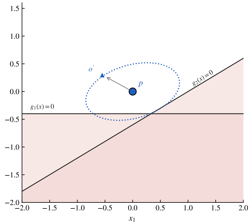
Subsequent generation: feasible sample from C'
