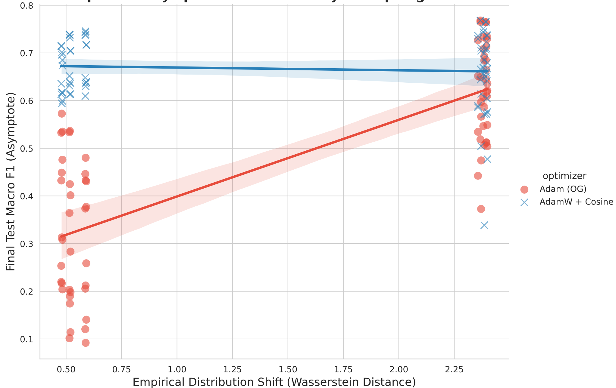
Adaptation Asymptote: Final Recovery vs. Topological Shift
