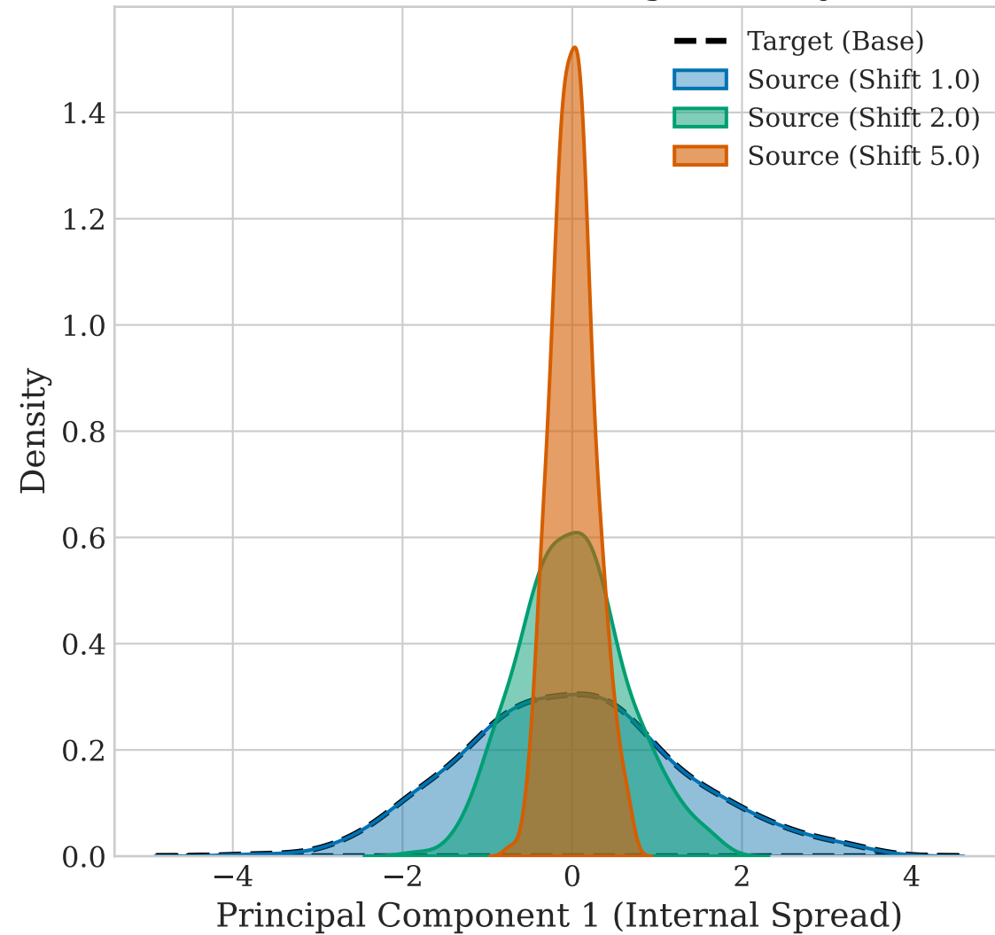
Covariate Shift (Single Family)
