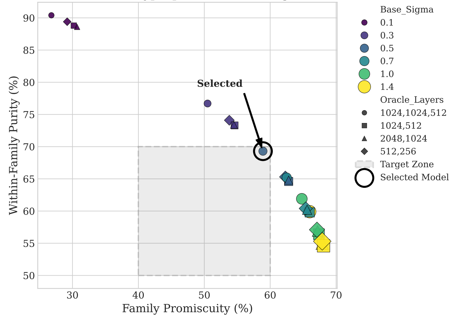
Oracle Hyperparameter Tuning
