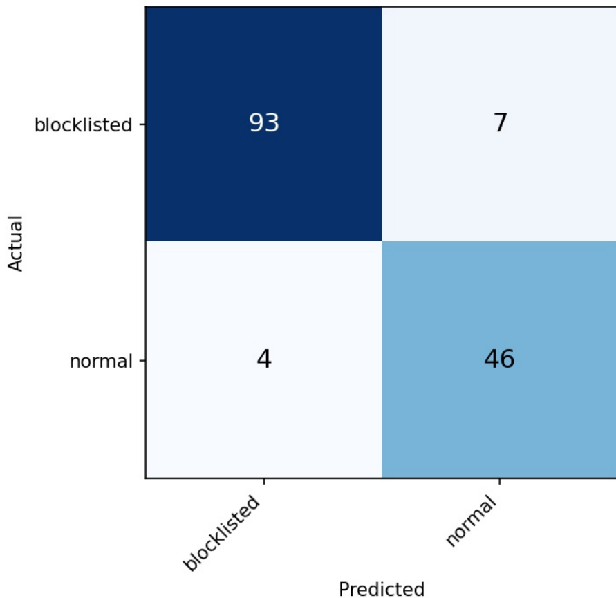
Confusion Matrix — RandomForest (Best)
