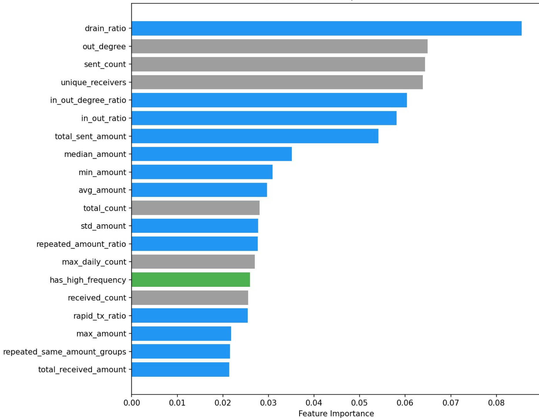
RandomForest — Top 20 Features
