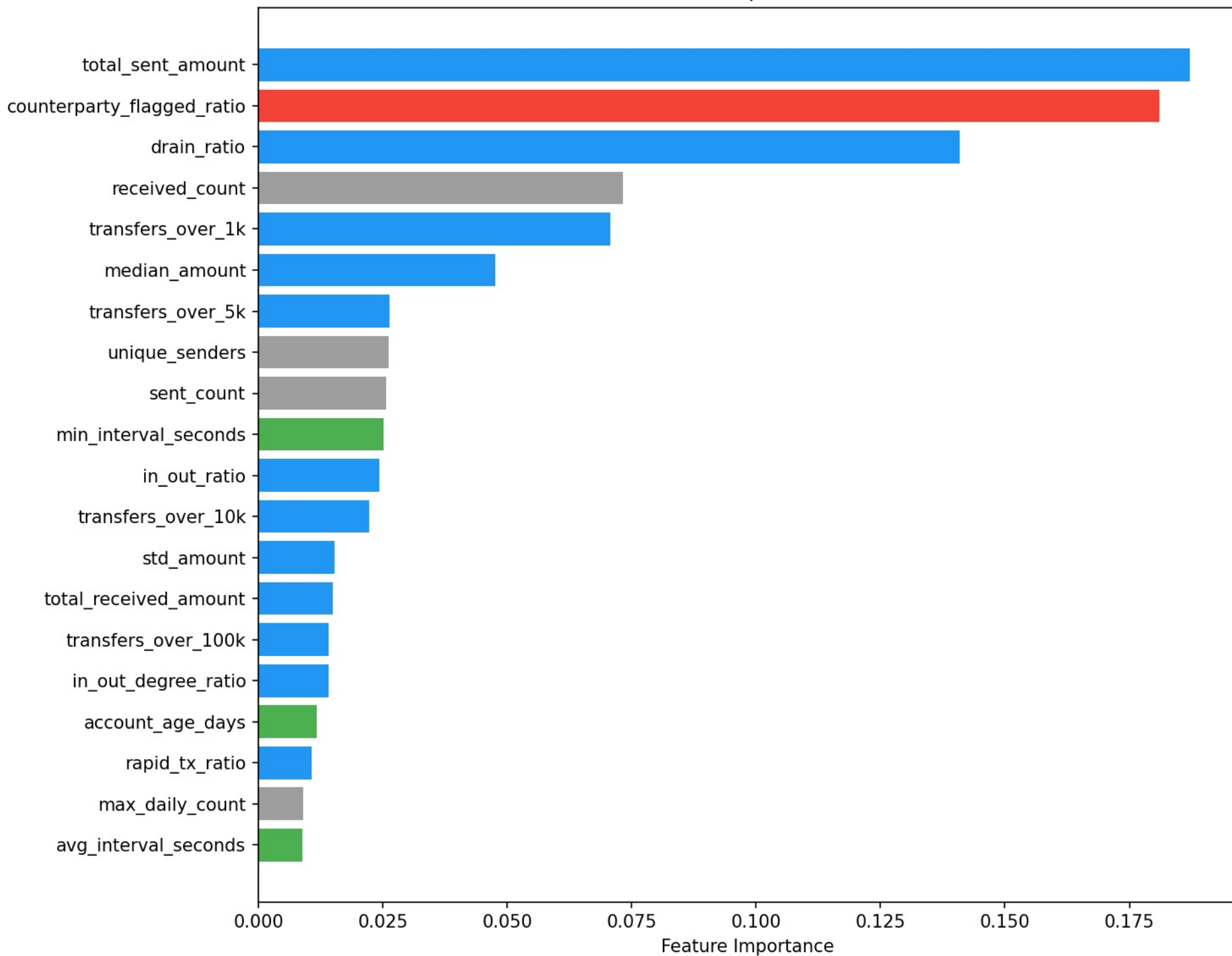
XGBoost — Top 20 Features
