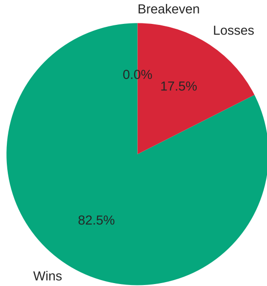
Win/Loss Distribution
