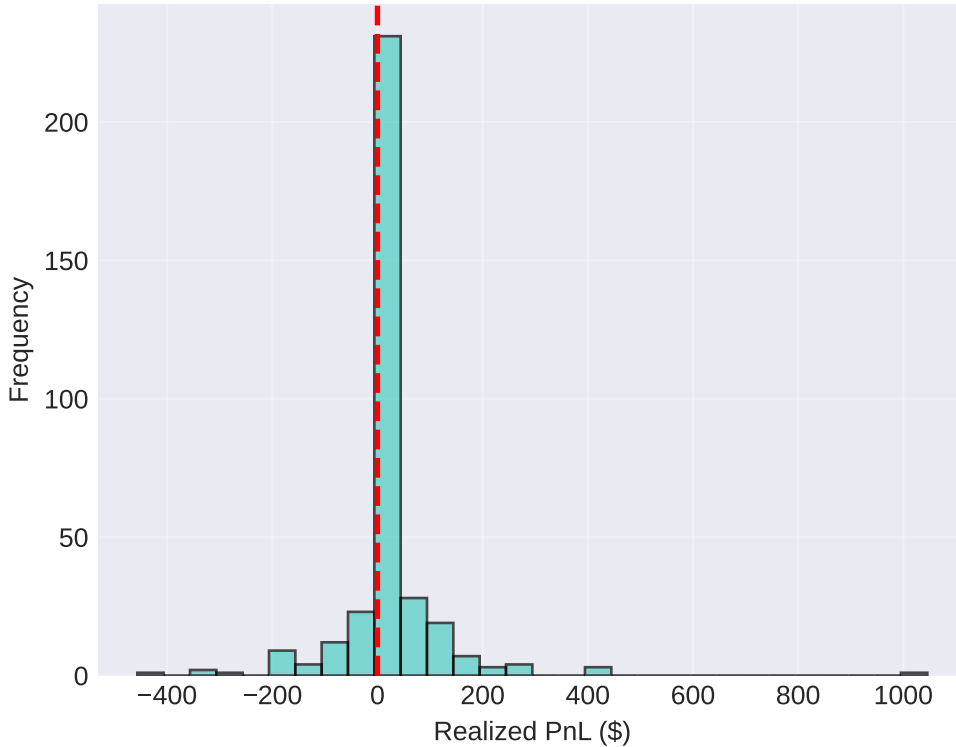
PnL Distribution
