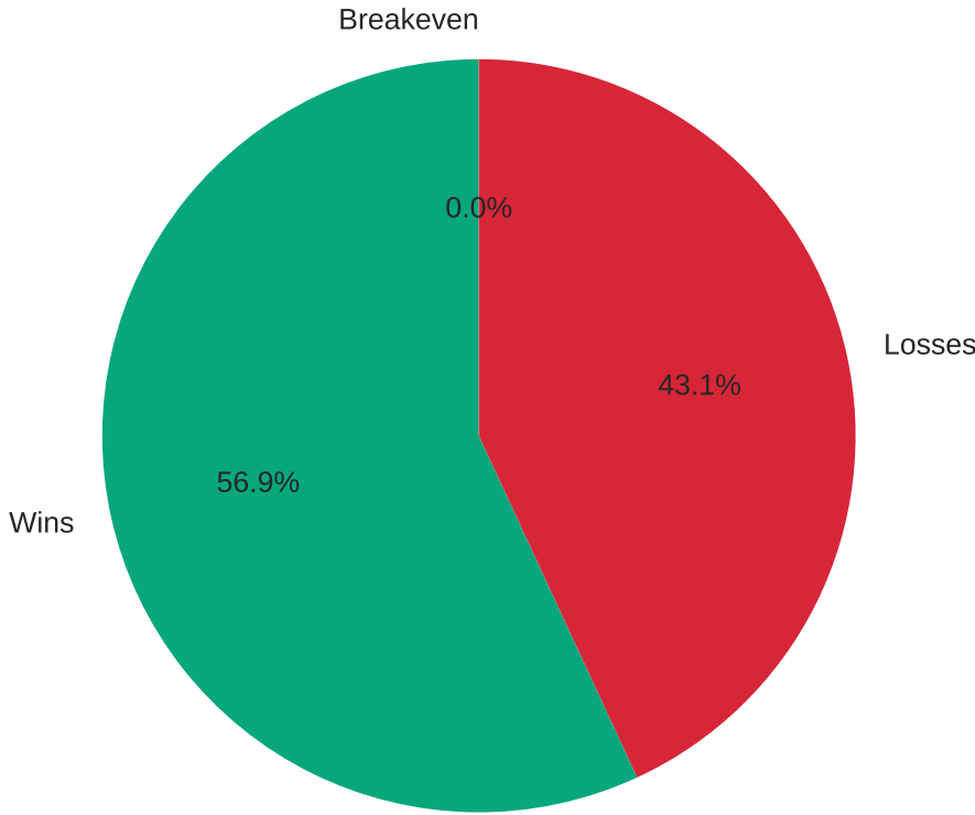
Win/Loss Distribution
