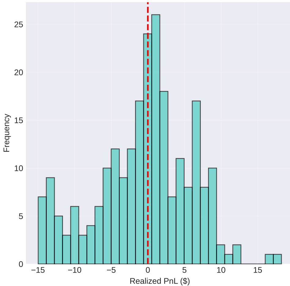
PnL Distribution
