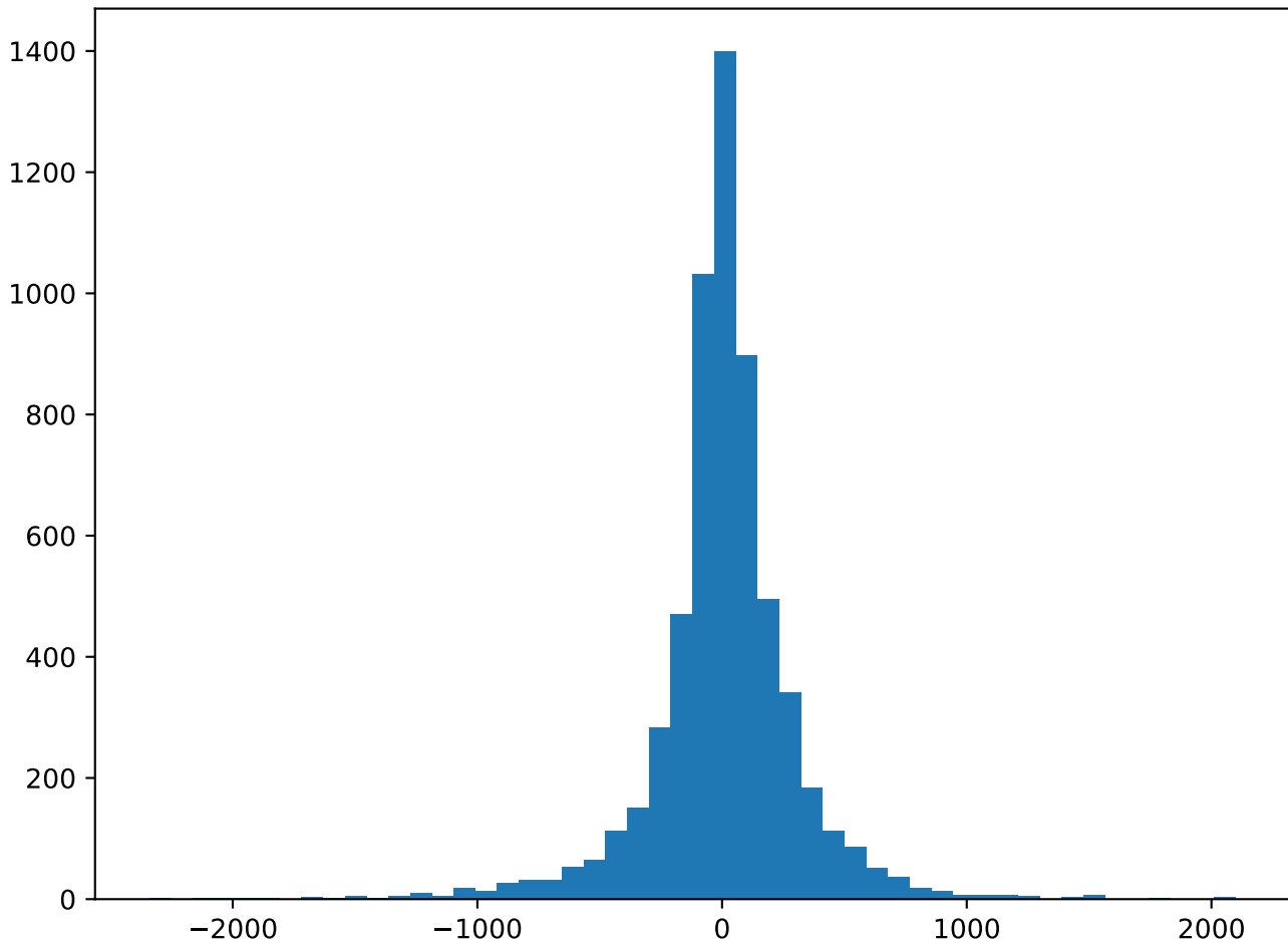
Test Histogram
