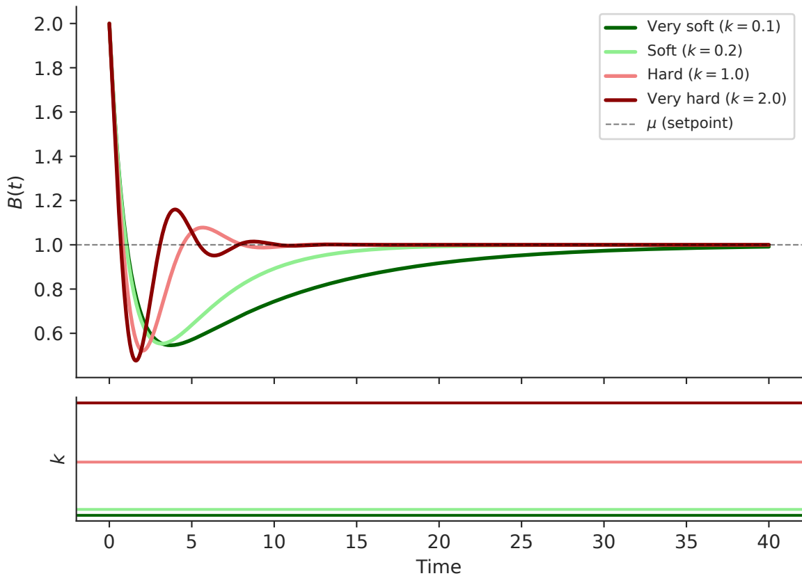
B converges to \mu for any fixed spring constant
