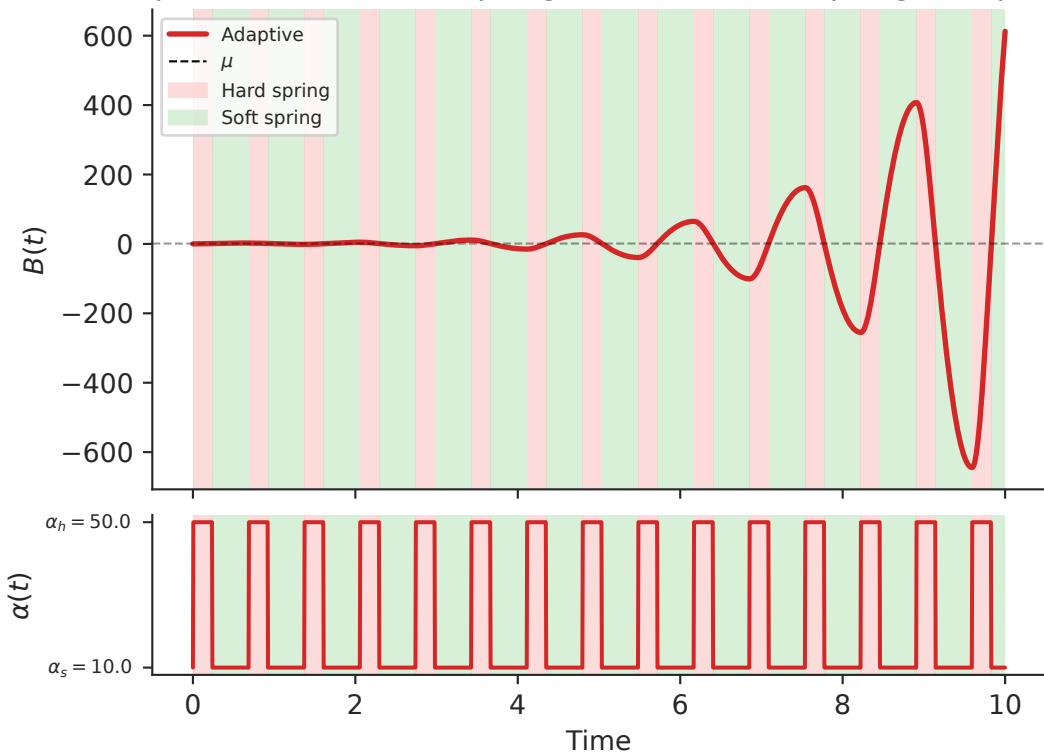
F) Adaptive control: hard spring when still, soft spring at equilibrium
