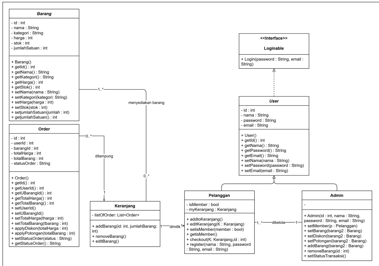
Class Diagram perangkat lunak Grow and Cheers
