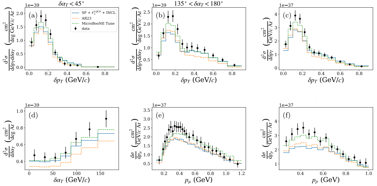
Figure 1: The most theory-driven GENIE configuration SF + F_A^{\text{LQCD}} + \text{INCL} (blue) compared with the AR23 (orange) and MicroBooNE (green) reference tunes on the MicroBooNE CC1 \mu 1p / CC1 \mu Np argon cross sections (black points). Panels: (a) \delta p_T for \delta\alpha_T < 45^\circ and (b) for 135^\circ < \delta\alpha_T < 180^\circ (two slices of the 2D \delta p_T – \delta\alpha_T measurement); (c) \delta p_T ; (d) \delta\alpha_T ; (e) p_\mu ; (f) p_p . Both reference tunes are drawn dashed. With INCL FSI the SF + F_A^{\text{LQCD}} prediction sits below the data around the \delta p_T peak and gives the largest \chi^2/\text{ndf} of the three in the 2D \delta p_T – \delta\alpha_T , \delta p_T and p_p distributions (see Table 1).
