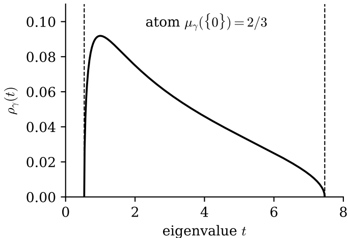
Marchenko-Pastur spectrum, \gamma = 3
