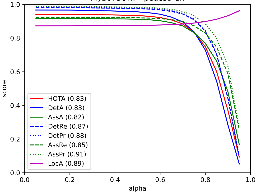
MyBoTSORT - pedestrian
