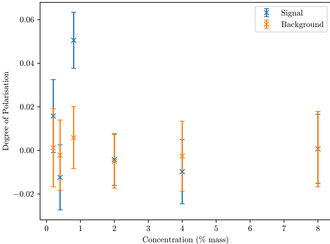
Latex Vertical Illumination Degree of Polarisation
