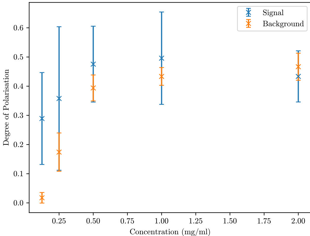
Dithered TiO 2 Horizontal Illumination Degree of Polarisation
