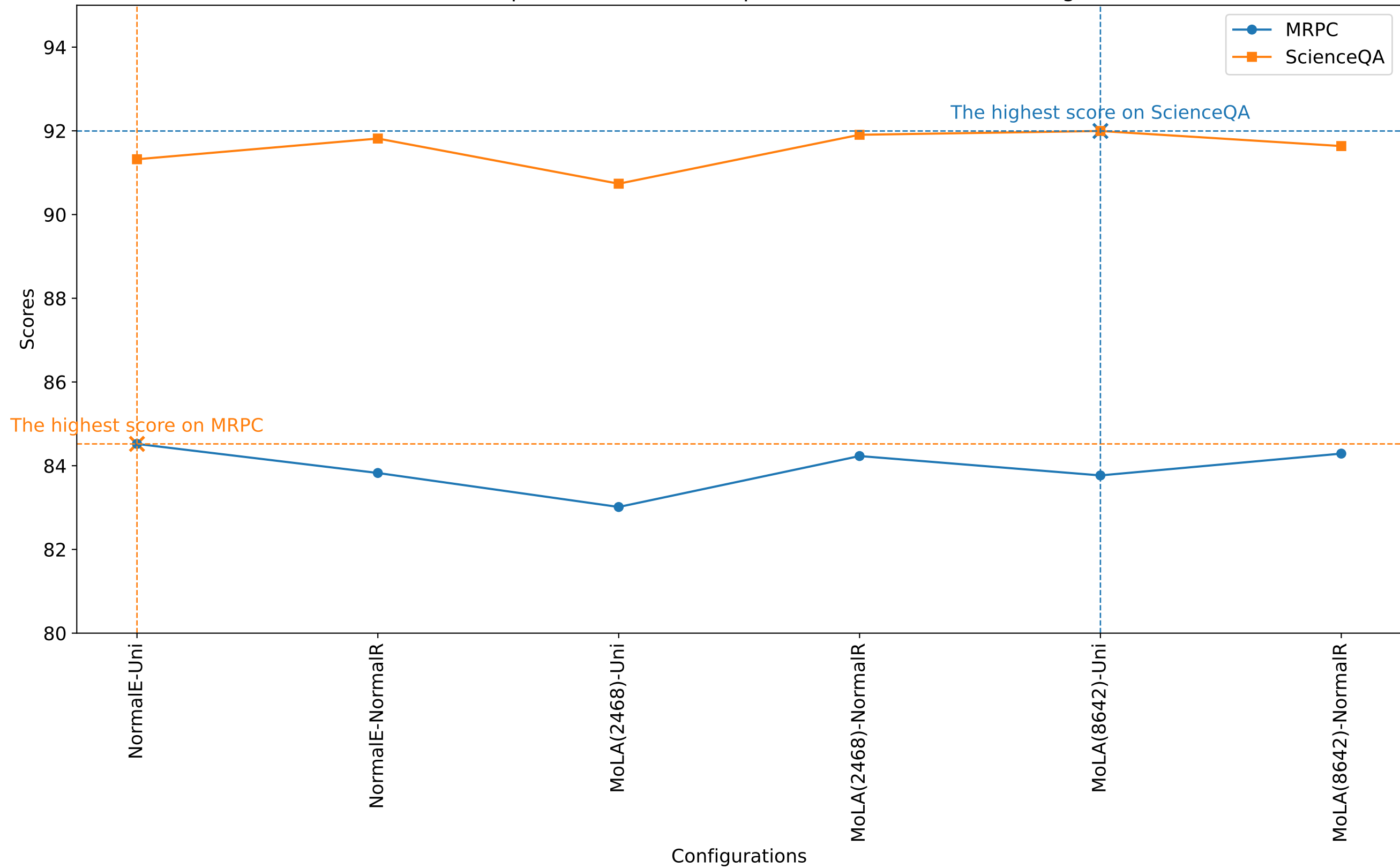
Performance Comparison Across 16 Expert Number and Rank Configurations
