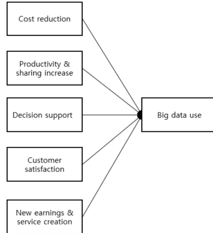
Fig. 2. Research Model
