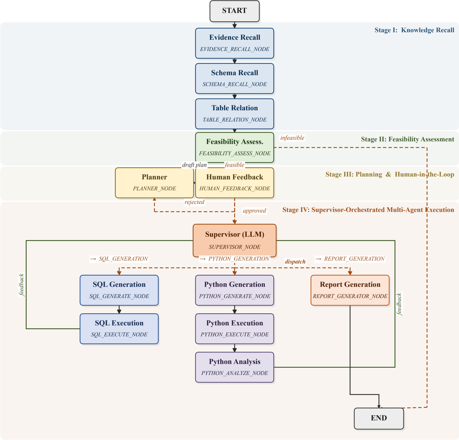
Fig. 1. End-to-End Multi-Node Agent Orchestration Graph of the Data-Agent Backend
